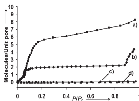
Figure 2. Adsorption profile of a) \text{H}_2\text{O} (squares), b) MeOH (diamonds), c) MeCN (circles), and d) EtOH (triangles) of 1a at 298 K.
